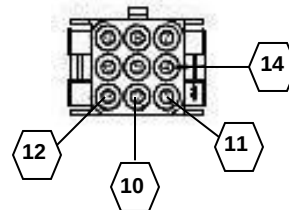
VIEW C – REAR OF LAD PLUG
