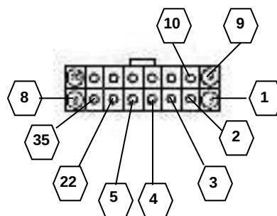
VIEW B – REAR OF CONTROLLER CONNECTOR
