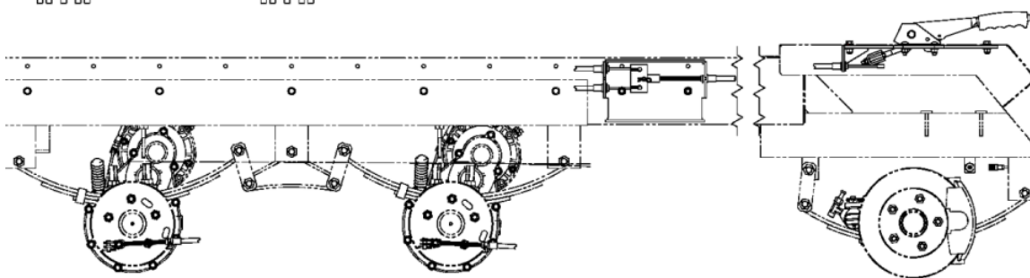
PARKING BRAKE, MVP-L HYD6, STD POSITION
