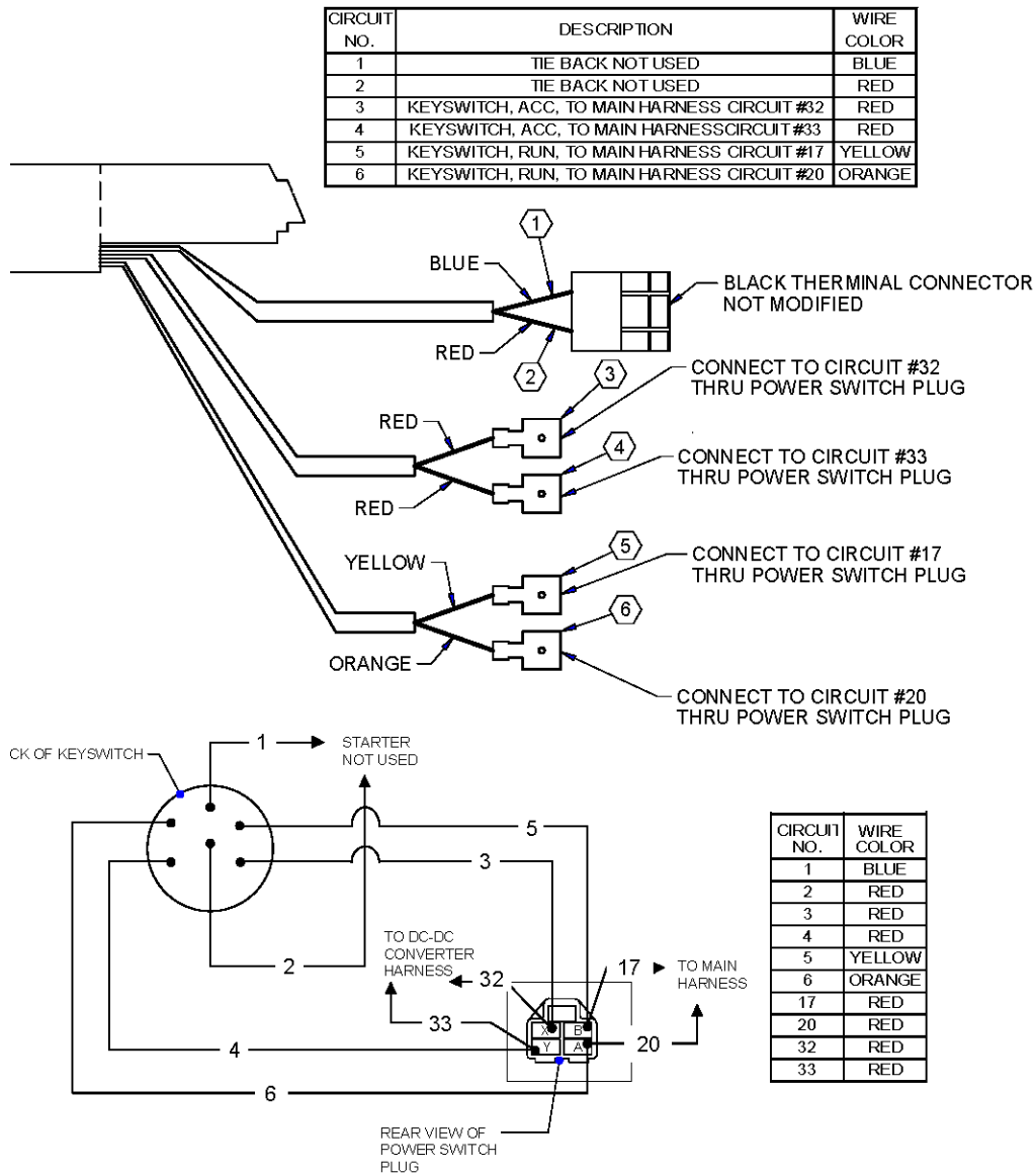
SCHEMATIC DIAGRAM
