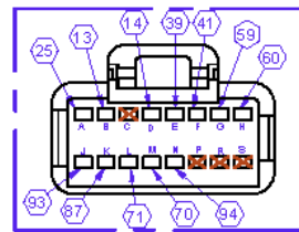
DETAIL I
