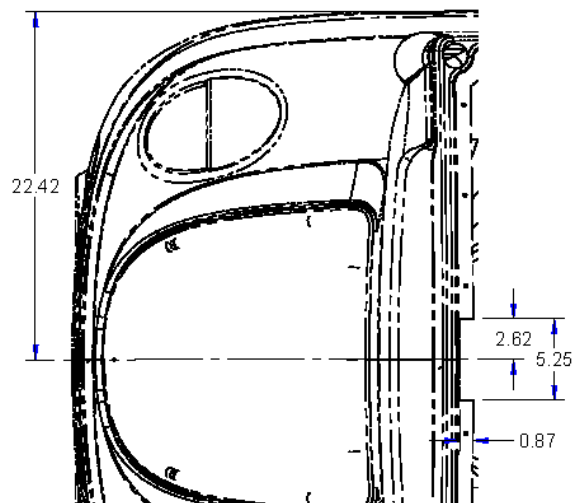
MAKE CUTOUT IN COWL AS SHOWN
