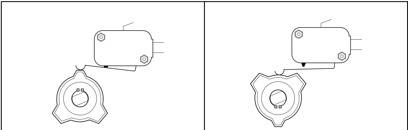
Figure 19 Neutral Lockout – Maintenance Position
