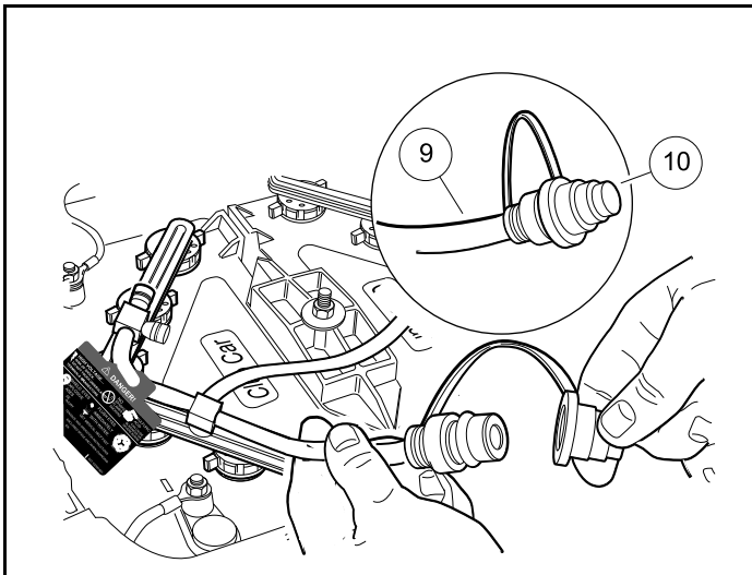
Figure 32 Dust Cap
