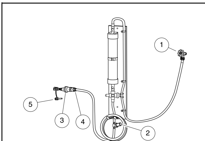
Figure 30 Connecting Hose with Filter to Water Source
