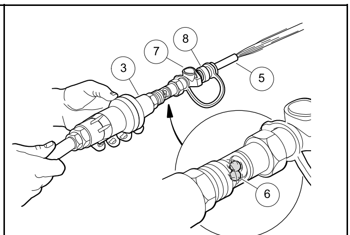
Figure 31 Checking the Water Flow Rate
