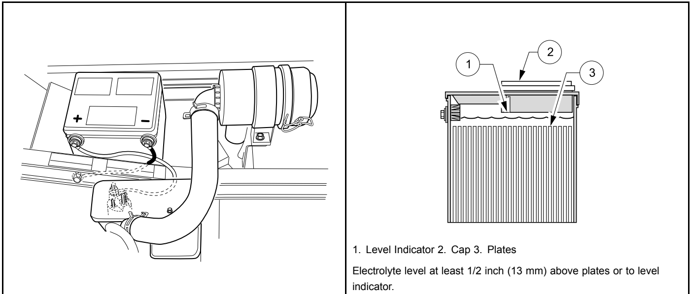
Figure 16 Gasoline Vehicle Battery
