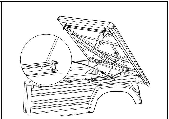
Figure 13 Prop Rod
