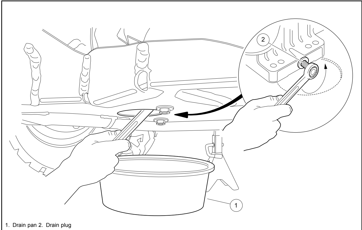
Figure 19 Engine Oil Drain Plug and Pan
