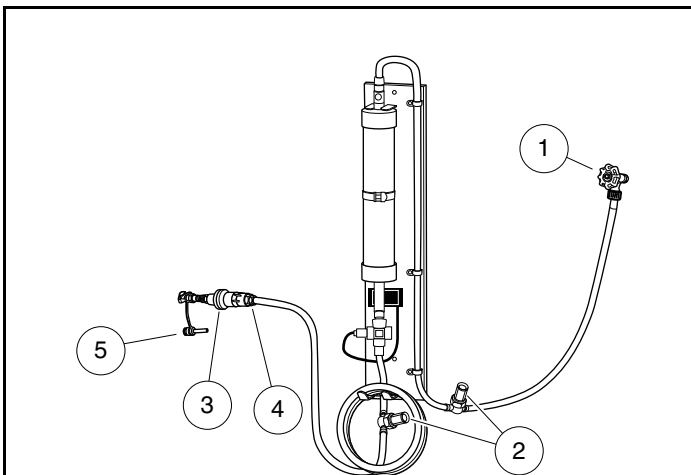
Figure 24 Connecting Hose with Filter to Water Source
