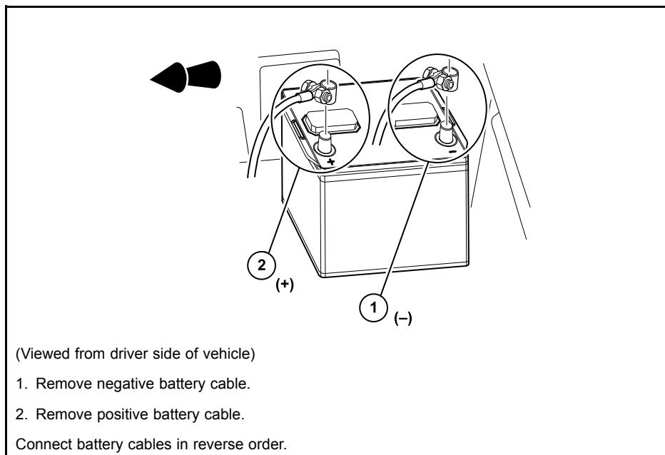
Figure 5 No Maintenance Battery: Battery Cable Removal-Gasoline Vehicles
