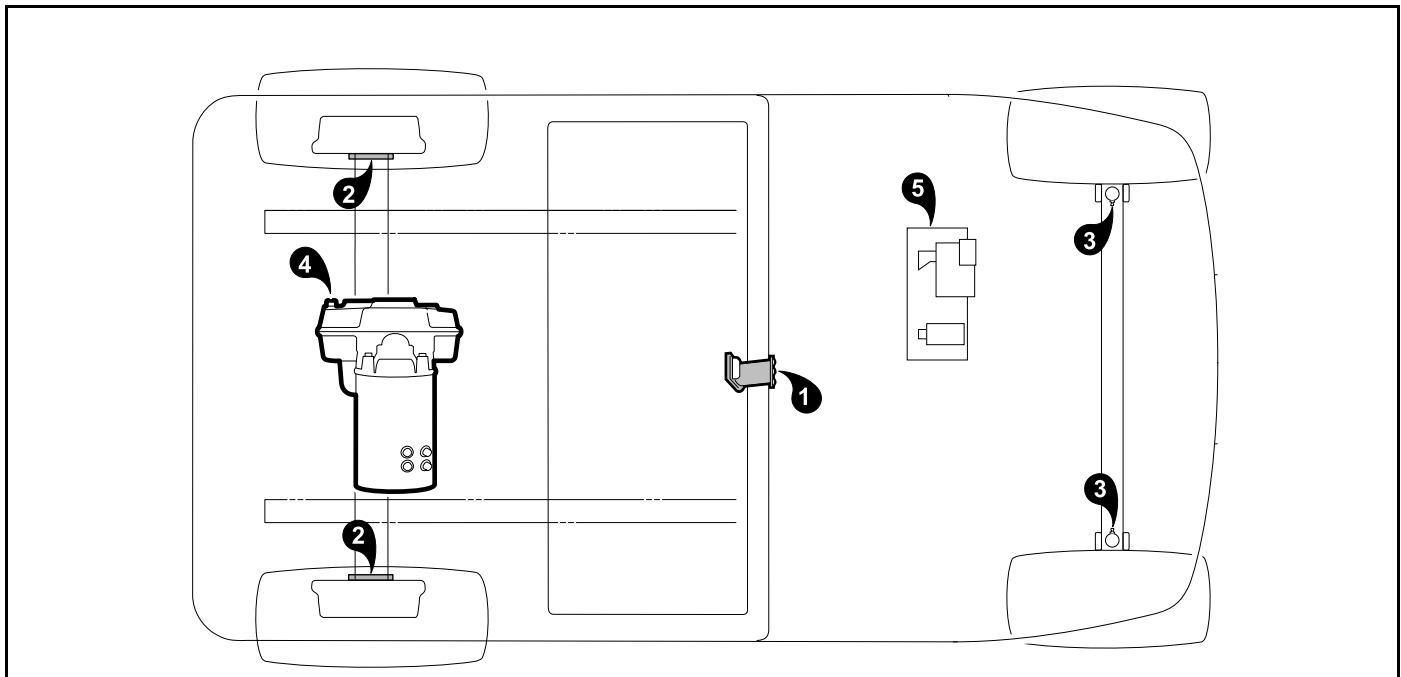
64.eps Figure 21 Lubrication Points – Electric Vehicles
